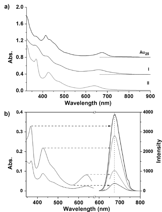
Figure 2. a) UV/Vis spectrum of \text{Au}_{25} , I , and II , the inset is a photo of the cluster solutions. b) photoluminescence properties of product II . PLE (—), UV/Vis (----). UV/Vis and excitation spectra (left), and emission spectra (right) at different excitation wavelengths, as indicated by arrows.
